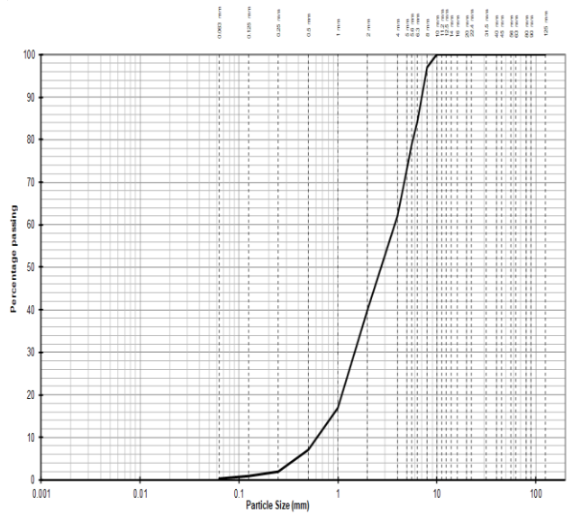
Typical Grading Graph - 0/10mm
