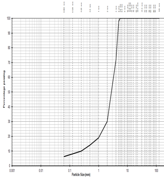
Typical Grading Graph - 0/4 mm
